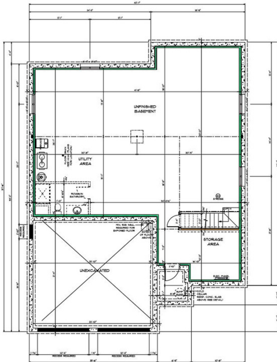
FOUNDATION PLAN SCALE 1/4"=1'-0"
